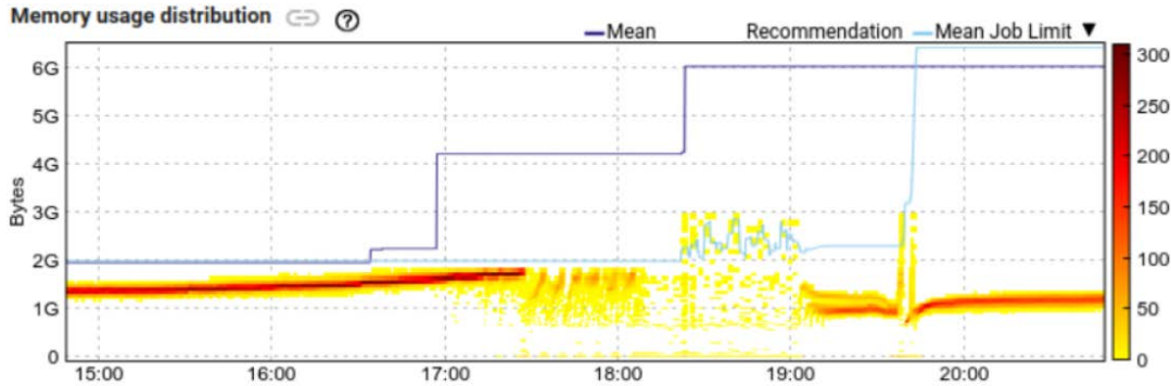
(b) A trace of a job using manually specified limits and with Autopilot running in simulation mode. A new roll-out had a memory leak that caused the memory usage to steadily increase. At about 17:30, the job's monitoring system started to page on-calls as the job started to OOM. It was not until 19:30 that the on-call dev/ops engineer managed to increase the job's memory limit (limit oscillations between 18:20 and 19:00 are an artifact of misalignment of time series data from the monitoring system). If the job had been Autopilot, it would probably not have OOMed as the automatically increased limits would have given dev/ops more time to discover the memory leak and roll back to the previous version of the binary.
