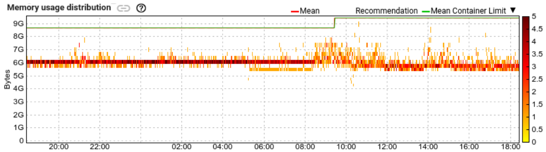
(a) A trace of an Autopilot job. Just after 8:00, some tasks started to exhibit an increased level of memory usage; Autopilot promptly increased the job's limit.
